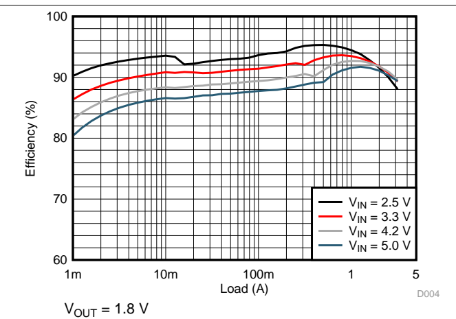
Figure 7. Efficiency
