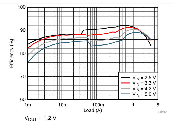
Figure 5. Efficiency
