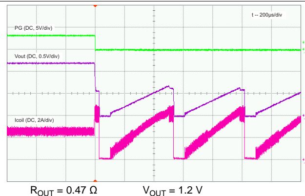
Figure 19. Output Short-Circuit Protection, Entry
