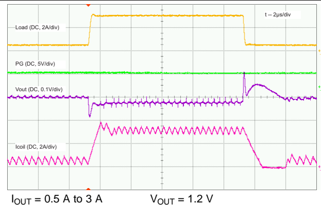
Figure 17. Load Transient
