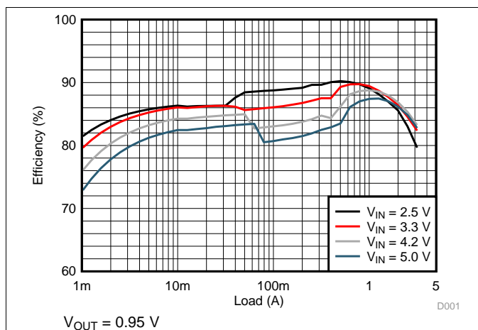
Figure 4. Efficiency
