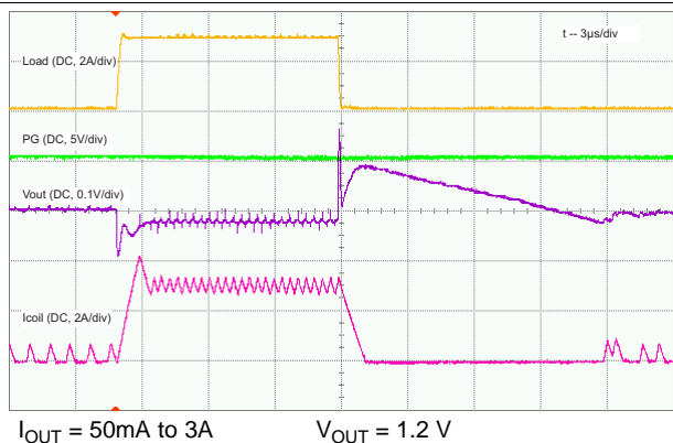
Figure 18. Load Transient
