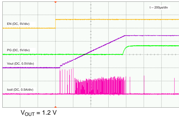
Figure 14. Start-Up without Load
