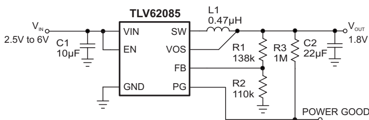
Figure 3. 1.8-V Output Voltage Application
