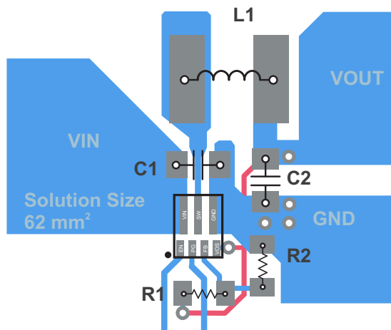
Figure 22. PCB Layout Recommendation
