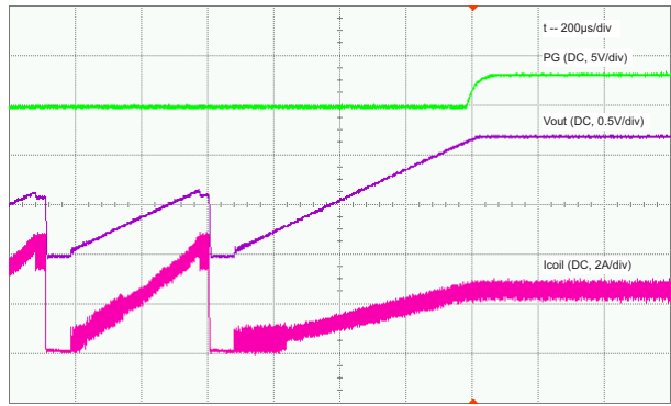
Figure 20. Output Short-Circuit Protection, Recovery
