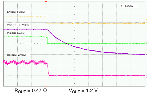
Figure 15. Shutdown with Load
