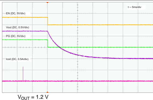
Figure 16. Shutdown without Load
