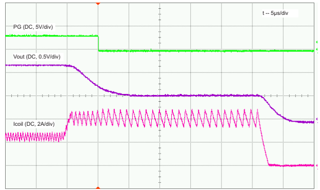
Figure 21. Output Short-Circuit Protection, HICCUP Zoom In
