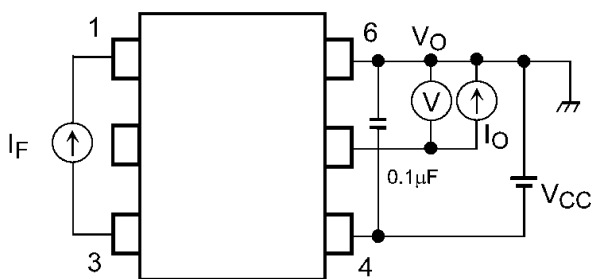
Fig. 13.1.1 IOBH Test Circuit
