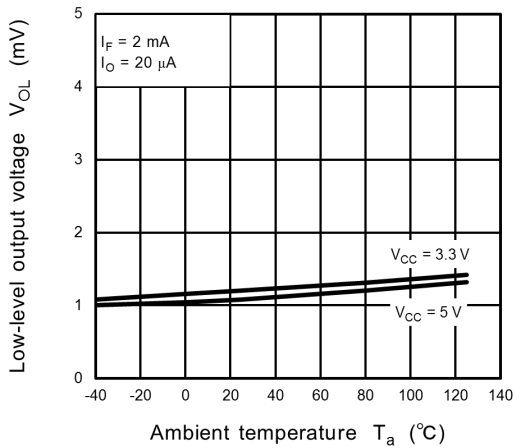
Fig. 13.2.3 V_{OL} - T_a
