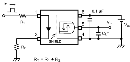
Fig. 13.1.5 Switching Time Test Circuit and Waveform
