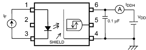
Fig. 13.1.4 IDDH Test Circuit
