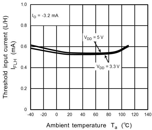
Fig. 13.2.9 I_{FLH} - T_a
