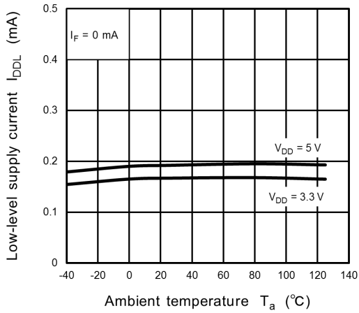
Fig. 13.2.7 I_{DDL} - T_a
