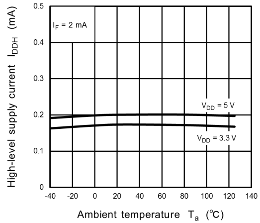
Fig. 13.2.8 I_{DDH} - T_a
