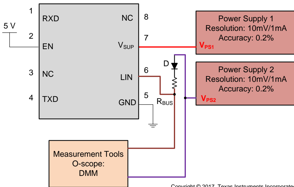
Figure 12. V_{SUP\_NON\_OP} Param 11
