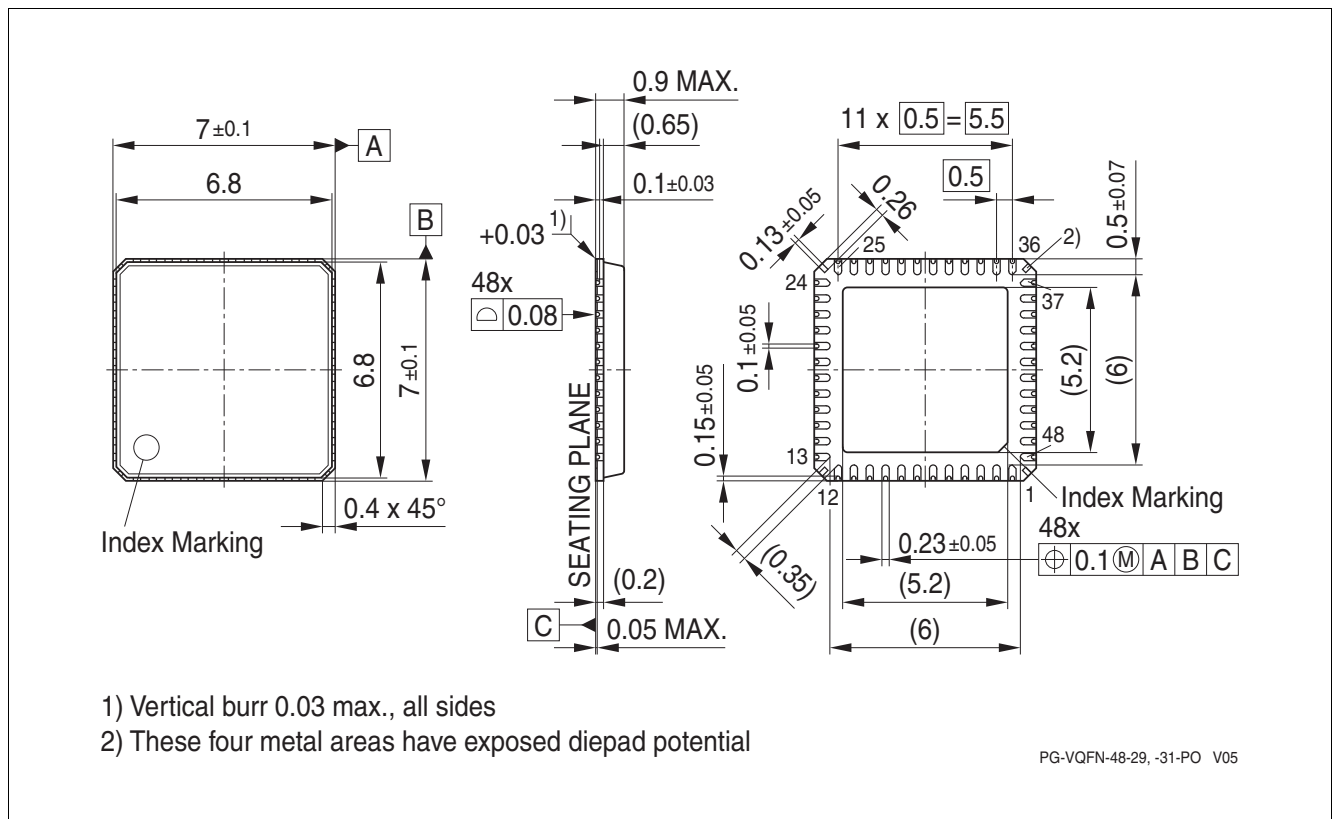
Figure 64 PG-VQFN-48 1)
