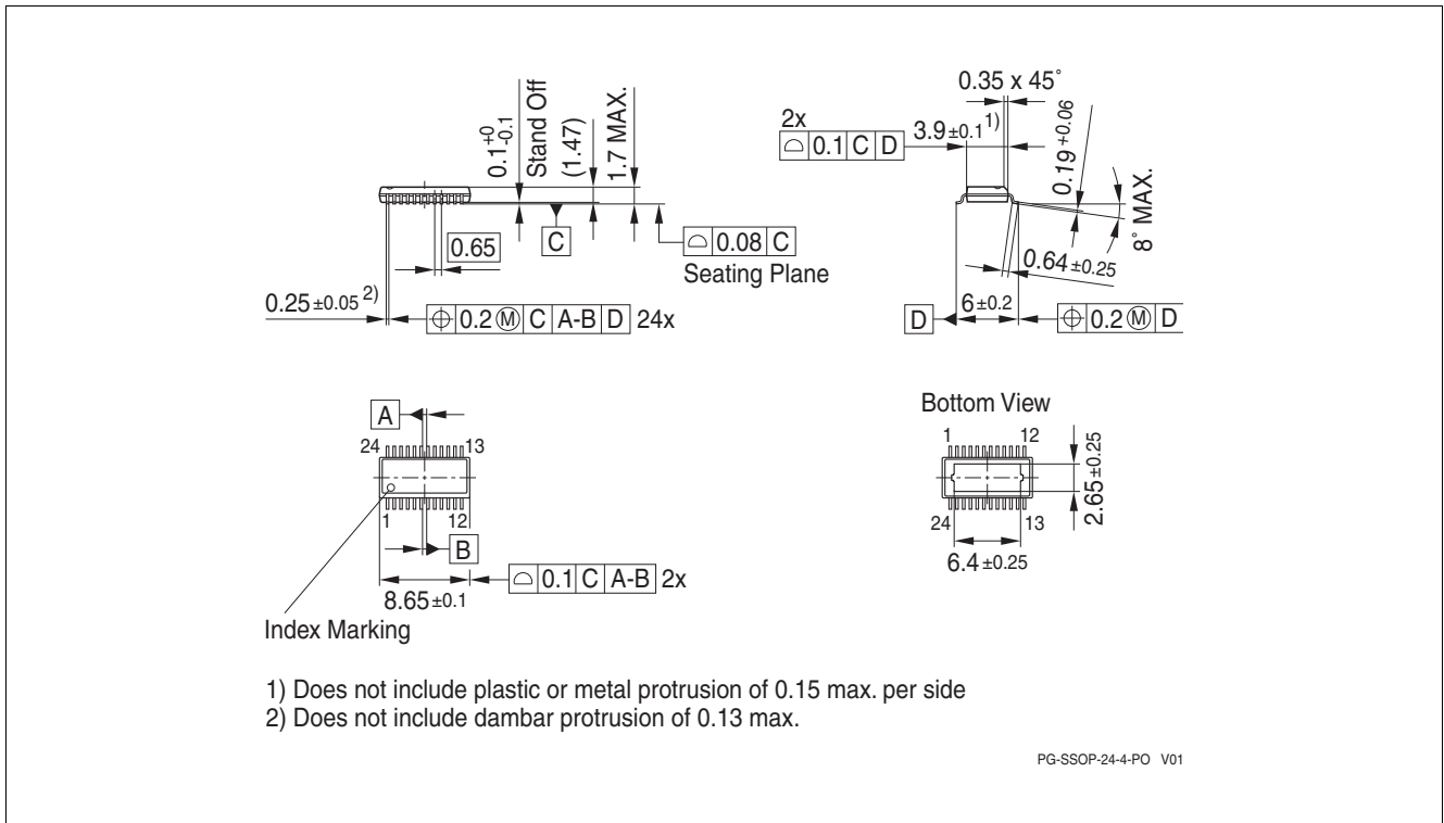
Figure 19 PG-SSOP24
