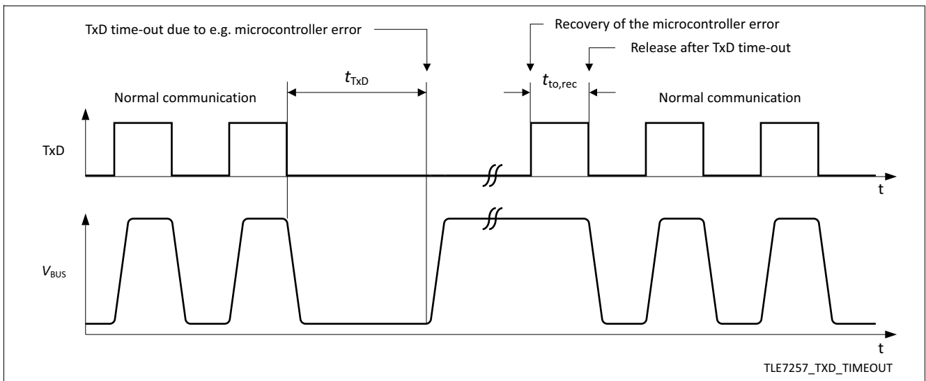
Figure 13 TxD time-out
