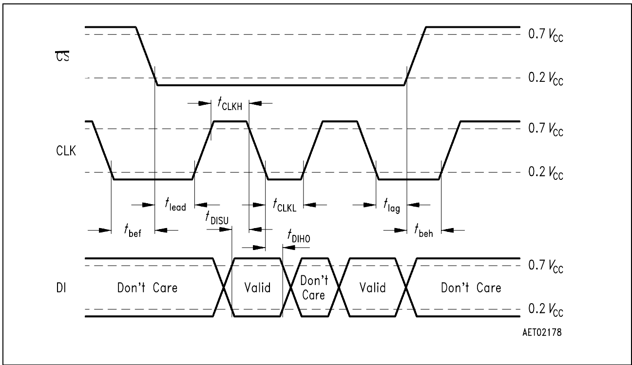
Figure 11 SPI-Input Timing
