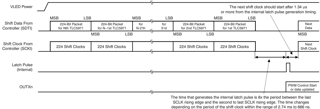
Figure 33. Data Packet and Display Start/Update Timing 1 (Internal Oscillator Mode)
