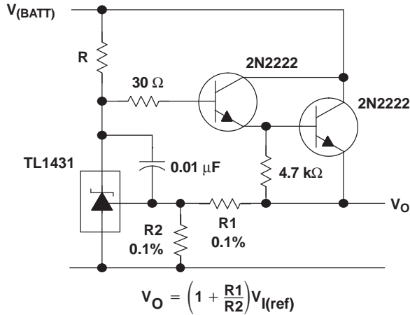
A. R should provide cathode current \geq 1 mA to the TL1431 at minimum V_{(\text{BATT})} . Figure 18. Precision High-Current Series Regulator
