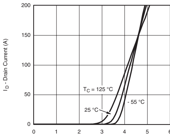
T_C = 125\text{ }^\circ\text{C} 25\text{ }^\circ\text{C} Transfer Characteristics
