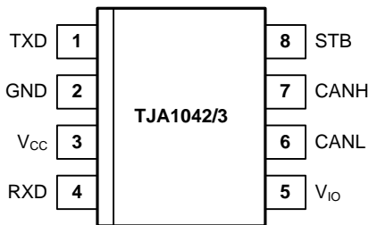
Fig 4. Pin configuration and short functional description of the TJA1042 and TJA1042/3
