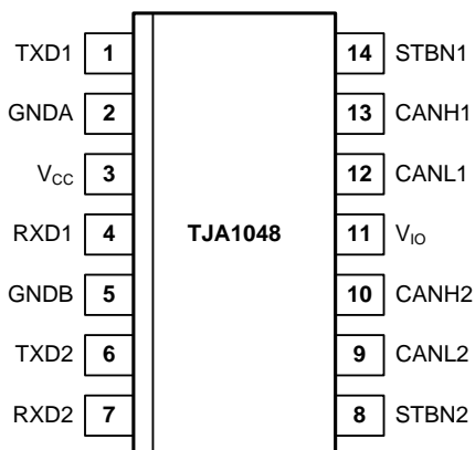
Fig 5. Pin configuration and short functional description of the TJA1048
