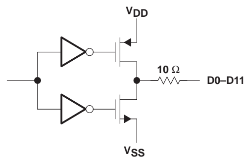
Figure 5. Digital Outputs
