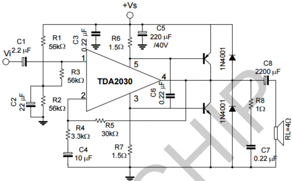
Fig. 1 Single supply high power amplifier
