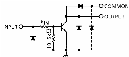
TD62597AFNG R_{IN}=2.7k TD62598AFNG R_{IN}=10.5k
