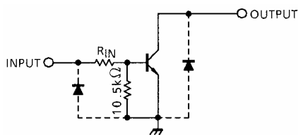
TD62593AFNG R_{IN}=2.7k TD62594AFNG R_{IN}=10.5k
