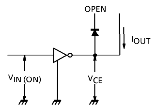
3. V_{IN(ON)}
