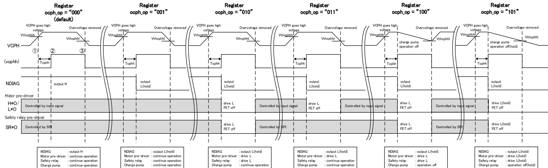
Fig. 7.5.3-b Timing chart for VCPH overvoltage
