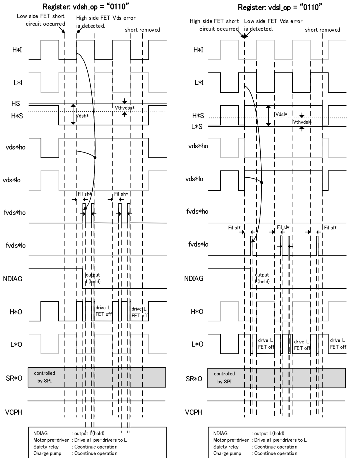
Fig. 7.5.8-h Timing chart for short-circuit detection (register vds l _op = vds h _op "0110")
