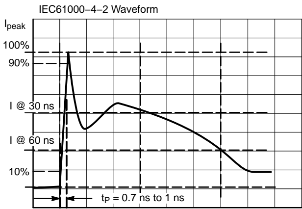
Figure 9. IEC61000-4-2 Spec
