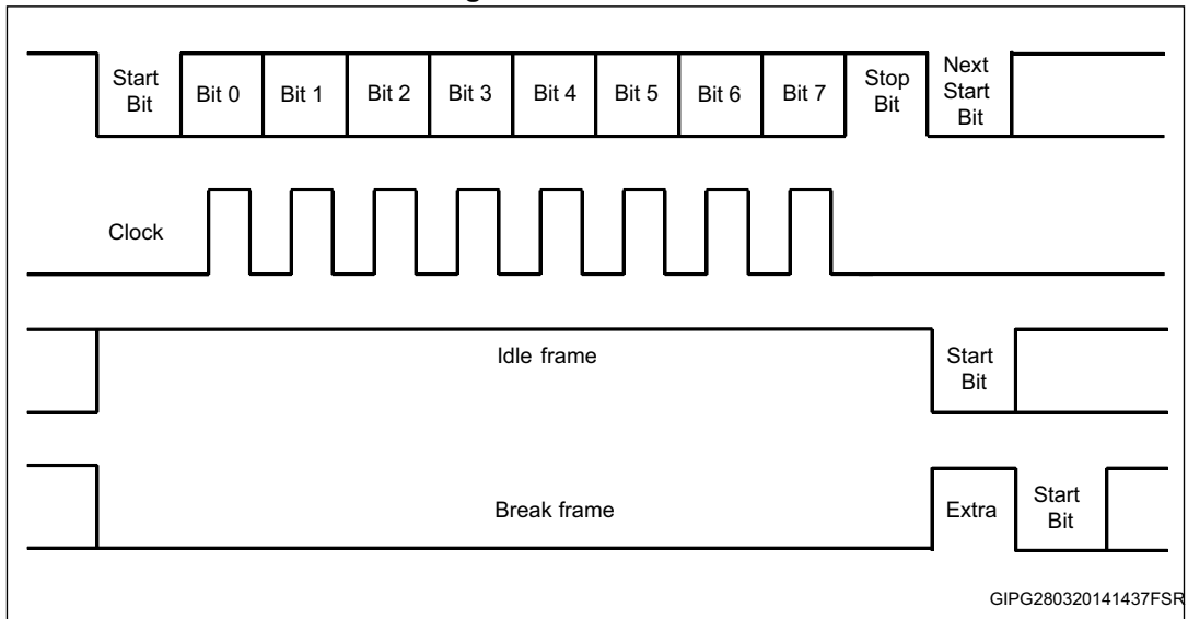
Figure 52. UART frame
