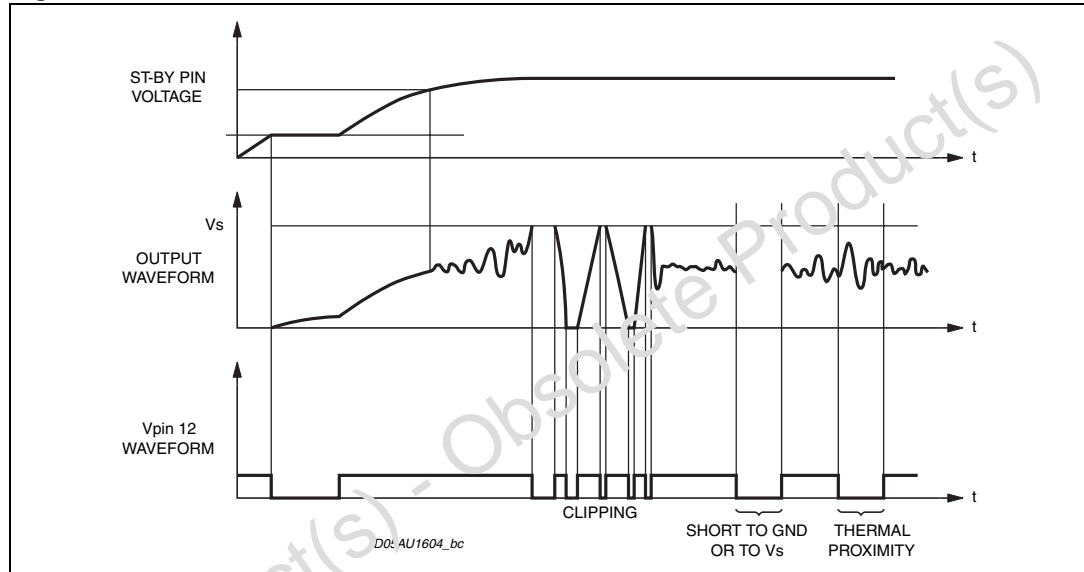
Figure 33. Waveforms
