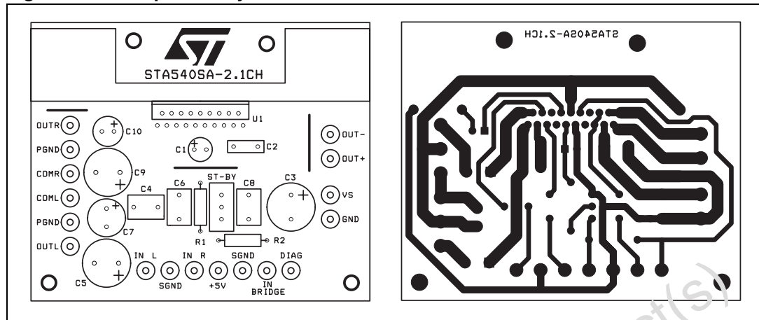
Figure 36. Component layout
