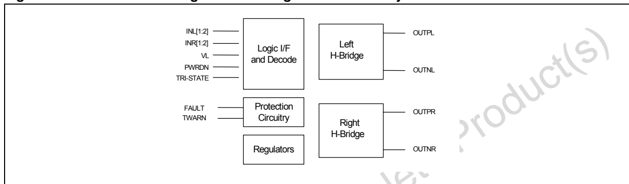
Figure 7. STA518A Block Diagram Full-Bridge DDX® or Binary Modes
