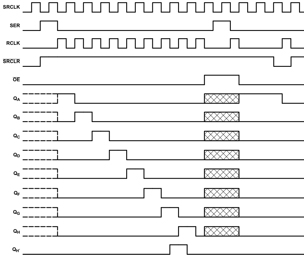
Figure 6-1. Timing Diagram
