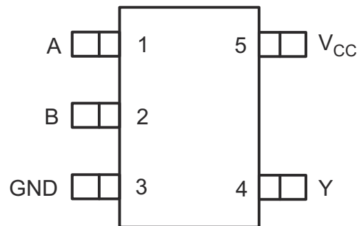
Figure 5-1. SN74LV1T32-Q1 DCK Package, 5-Pin SC-70 (Top View)
