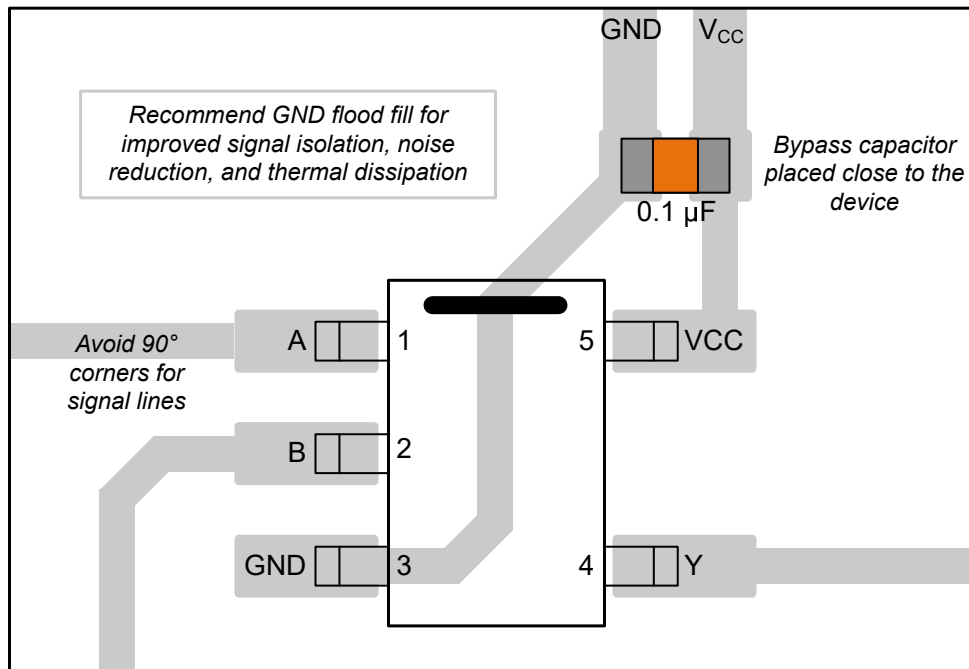
Figure 9-3. Example Layout for the SN74LV1T32-Q1
