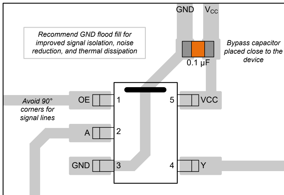
Figure 11-1. Example Layout for the SN74LV1T125-Q1
