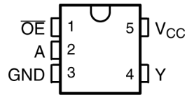
Figure 5-1. SN74LV1T125-Q1 DCK Package, 5-Pin SC70 (Top View)
