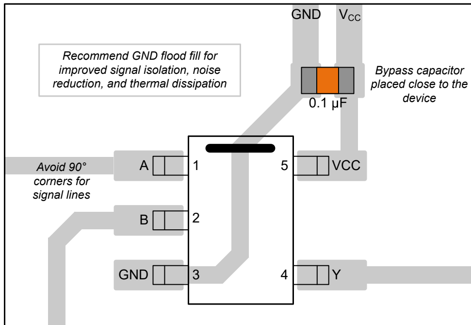
Figure 9-3. Example Layout for the SN74LV1T08-Q1
