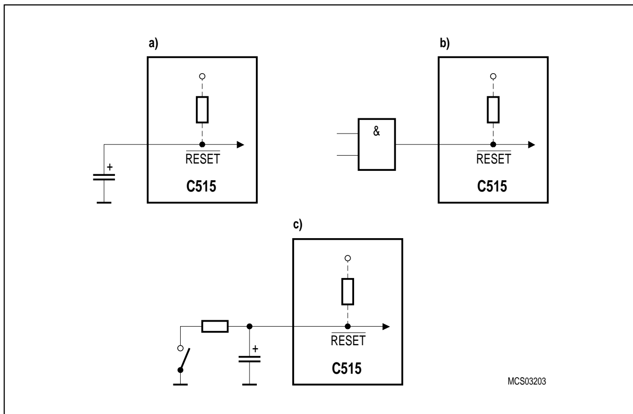
Figure 6 Reset Circuitries
