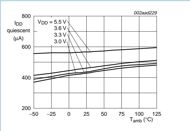
Fig 13. Typical I_{DD} quiescent current versus temperature and V_{DD} (conversion rate = 16 Hz)
