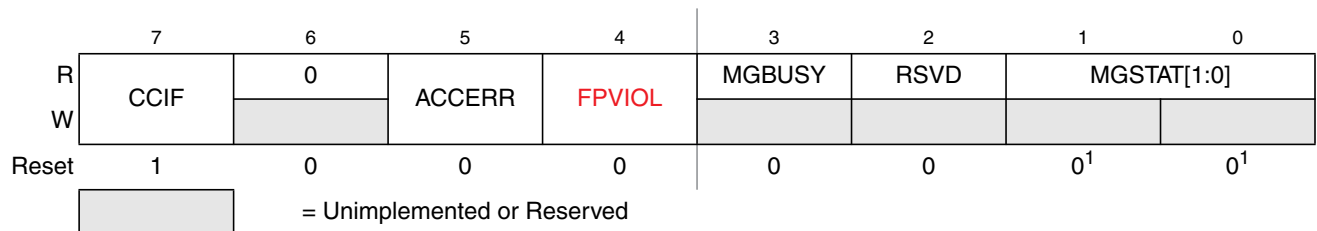
Figure 26-11. Flash Status Register (FSTAT)
