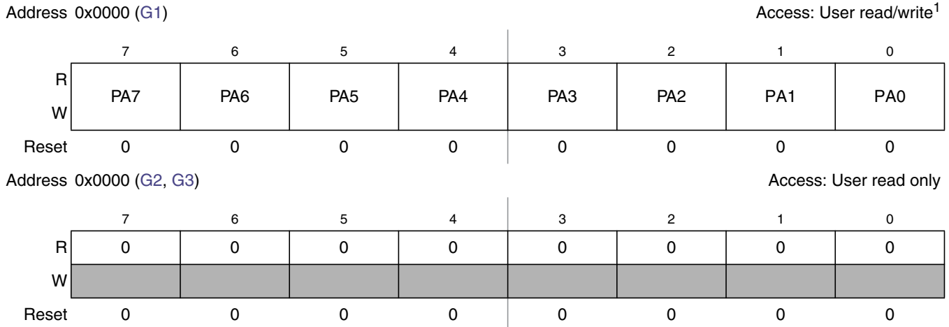
Figure 2-2. Port A Data Register (PORTA)
