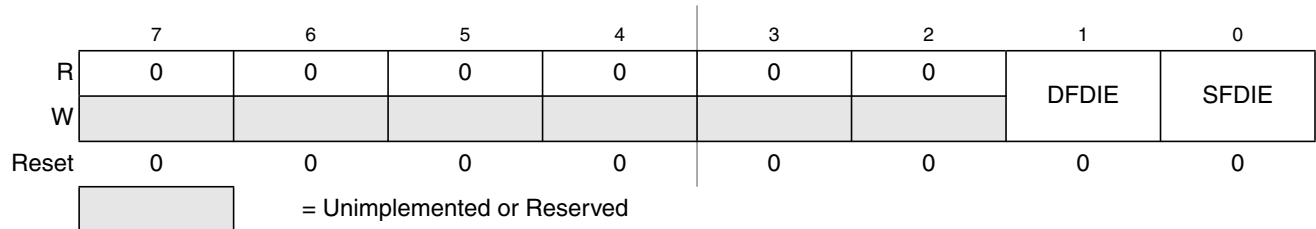
Figure 30-10. Flash Error Configuration Register (FERCNFG)
