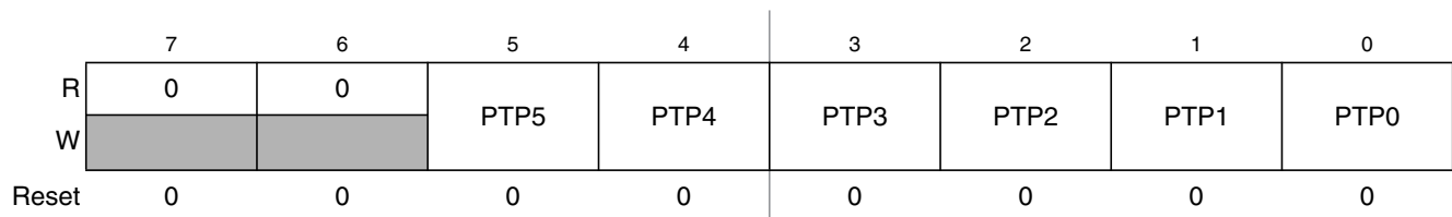
Figure 2-35. Port P Data Register (PTP)
