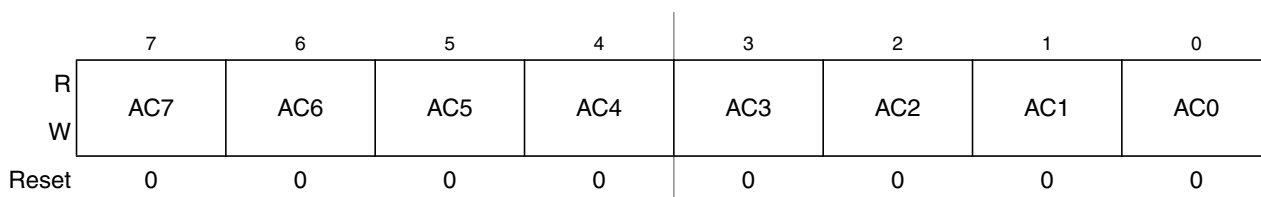
Figure 18-20. MSCAN Identifier Acceptance Registers (First Bank) — CANIDAR0–CANIDAR3
