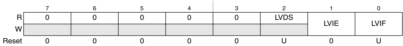
Figure 10-16. Low Voltage Control Register (CPMULVCTL)
