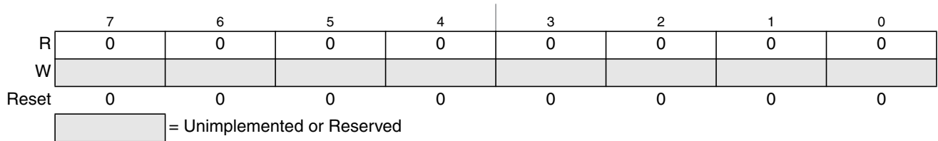
Figure 10-29. Reserved Register CPMUTEST2
