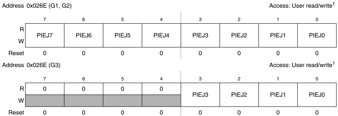
Figure 2-47. Port J Interrupt Enable Register (PIEJ)
