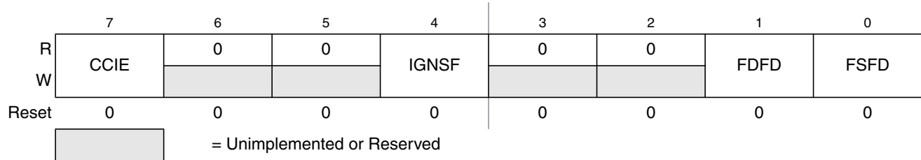
Figure 22-9. Flash Configuration Register (FCNFG)
