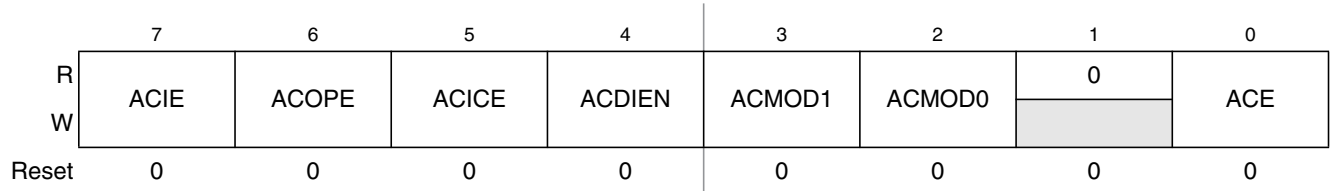
Figure 3-3. ACMP Control Register (ACMPC)
