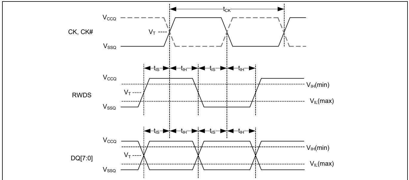
Figure 27 DDR input timing reference level
