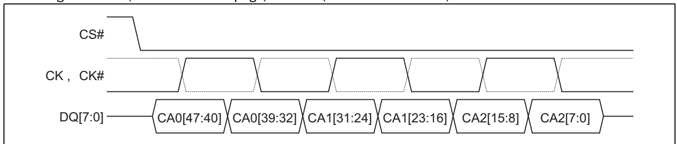
Figure 6 Command/address (CA) sequence [4-7]
