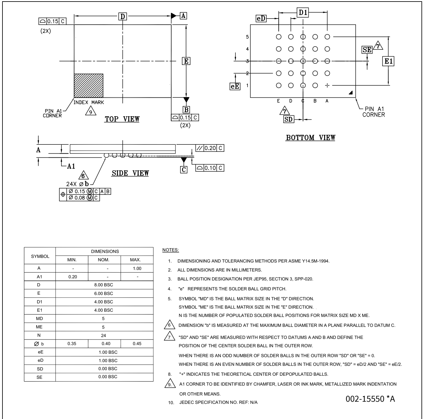
Figure 36 Fortified ball grid-array 24-ball 6 x 8 x 1.0 mm (VAA024)
