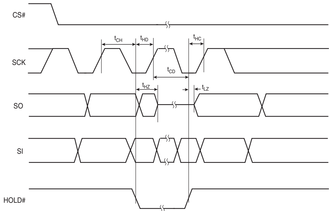
Figure 19.3 HOLD# Timing
