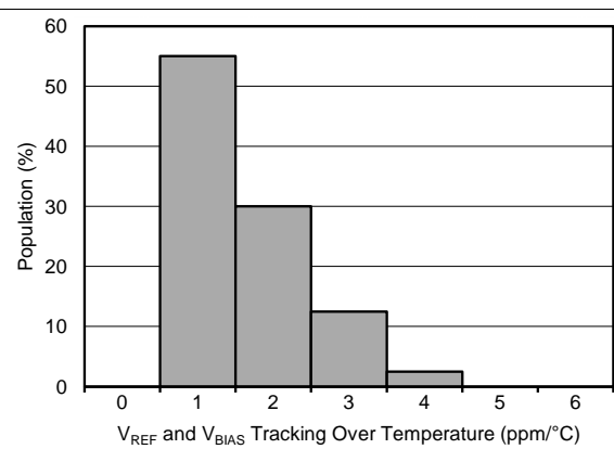
Figure 53. Distribution of V REF - 2 × V BIAS Drift Tracking Over Temperature
