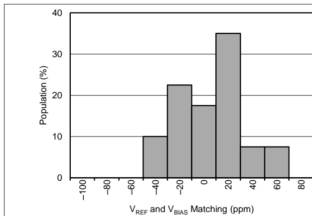
Figure 52. V REF - 2 × V BIAS Distribution (At T A = 25°C)
