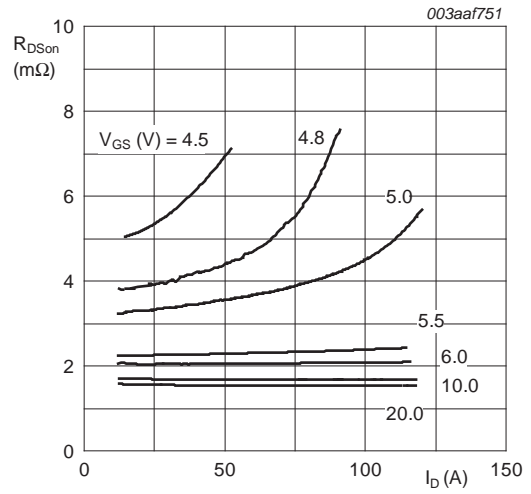
T_j = 25\text{ °C}
