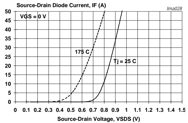
Fig 15. Source current as a function of source-drain voltage; typical values
