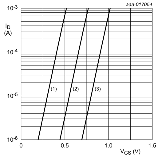
Fig. 7. Sub-threshold drain current as a function of gate-source voltage V_{DS} = 5 V T_j = 25 \text{ }^\circ\text{C} (1) minimum values (2) typical values (3) maximum values
