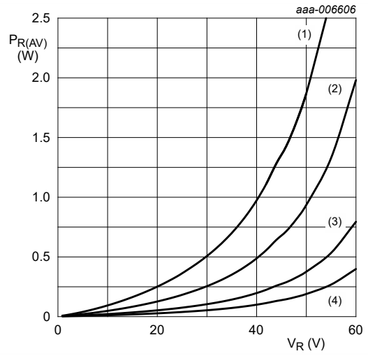
T_j = 125\text{ °C} (1) \delta = 1 (2) \delta = 0.5 (3) \delta = 0.2 (4) \delta = 0.1
