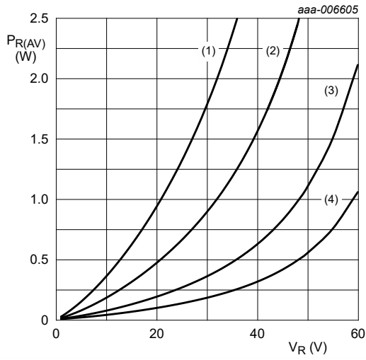
T_j = 150\text{ °C} (1) \delta = 1 (2) \delta = 0.5 (3) \delta = 0.2 (4) \delta = 0.1
