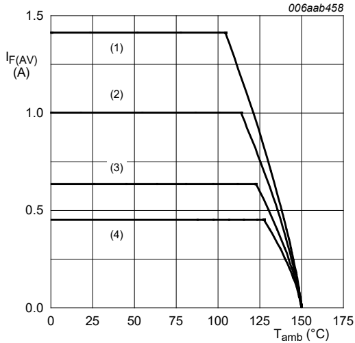
FR4 PCB, mounting pad for cathode 1 cm 2 T_j = 150\text{ }^\circ\text{C} (1) \delta = 1 ; DC (2) \delta = 0.5 ; f = 20\text{ kHz} (3) \delta = 0.2 ; f = 20\text{ kHz} (4) \delta = 0.1 ; f = 20\text{ kHz}
