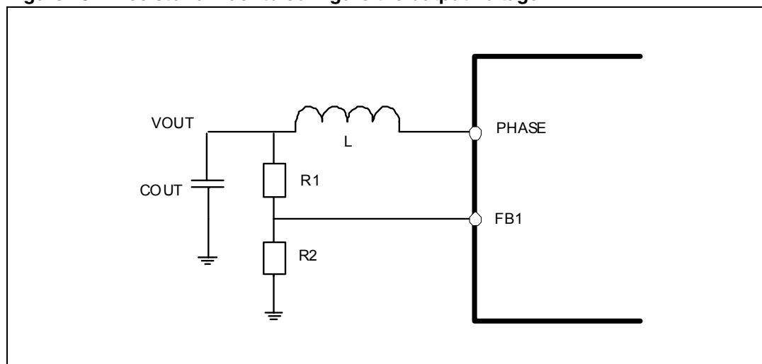
Figure 45. Resistor divider to configure the output voltage
