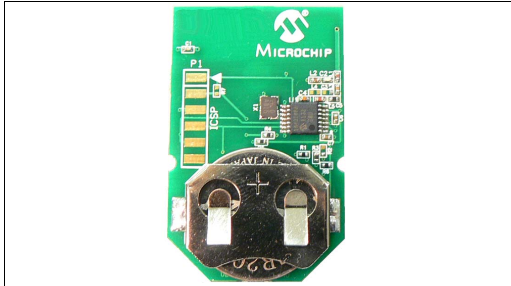
FIGURE 3-2: PCB TOP LAYER PHOTO
