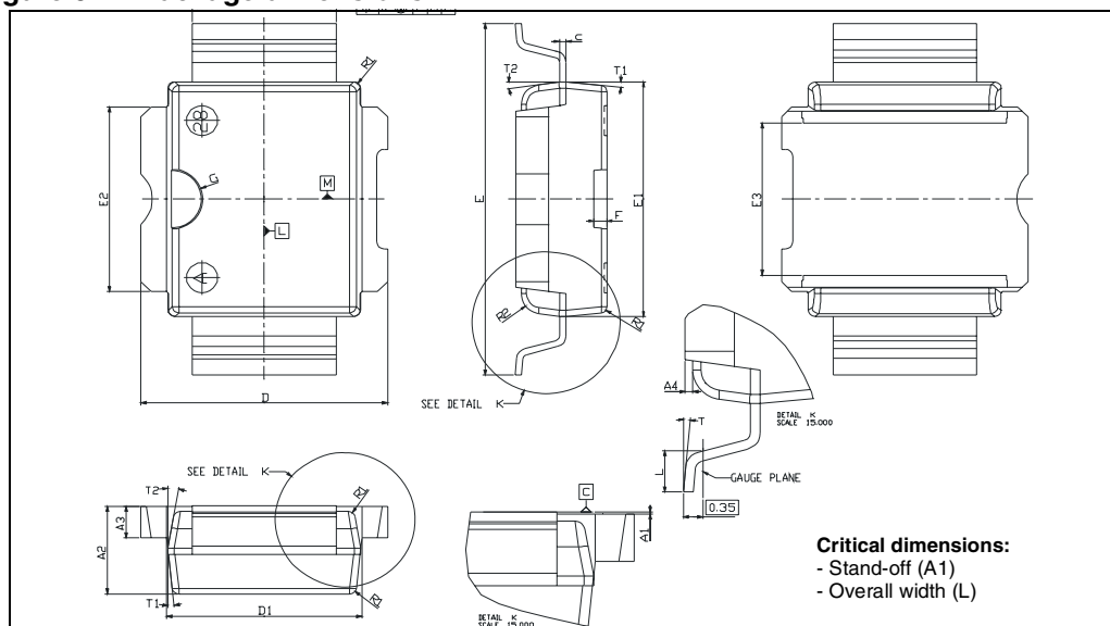
Figure 6. Package dimensions
