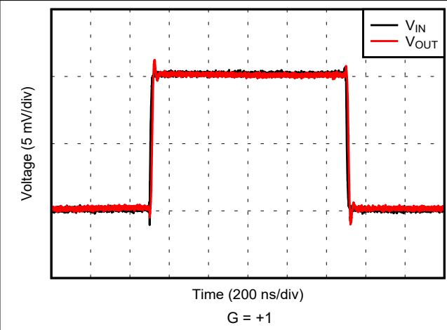
Figure 6-33. Small-Signal Step Response
