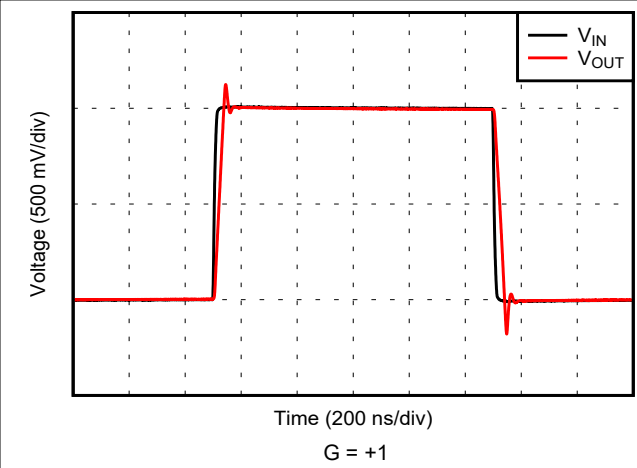
Figure 6-35. Large-Signal Step Response
