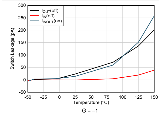
Figure 6-36. Switch Leakage Current vs Temperature
