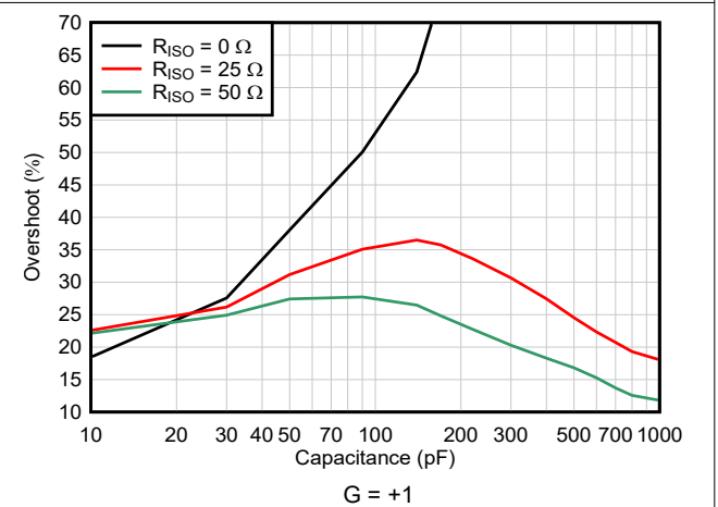
Figure 6-29. Small-Signal Overshoot vs Load Capacitance
