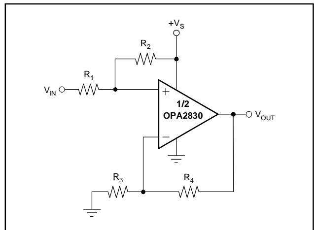
Figure 74. DC Level-Shifting
