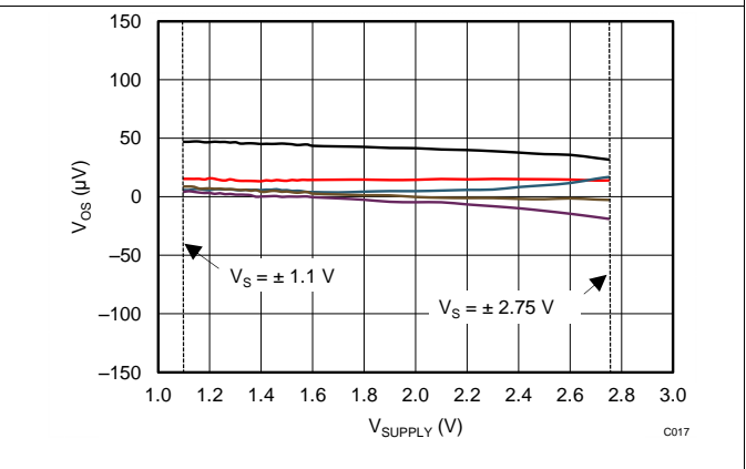
Figure 6. Offset Voltage vs Supply Voltage
