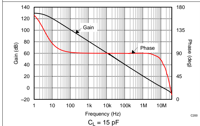
Figure 5. Open-Loop Gain and Phase vs Frequency
