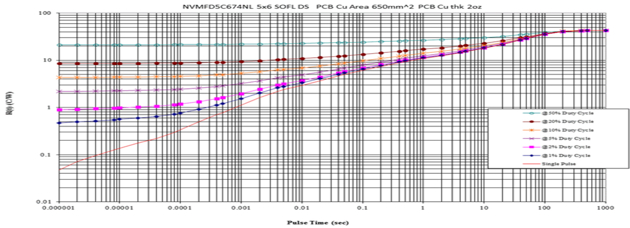
Figure 13. Thermal Characteristics
