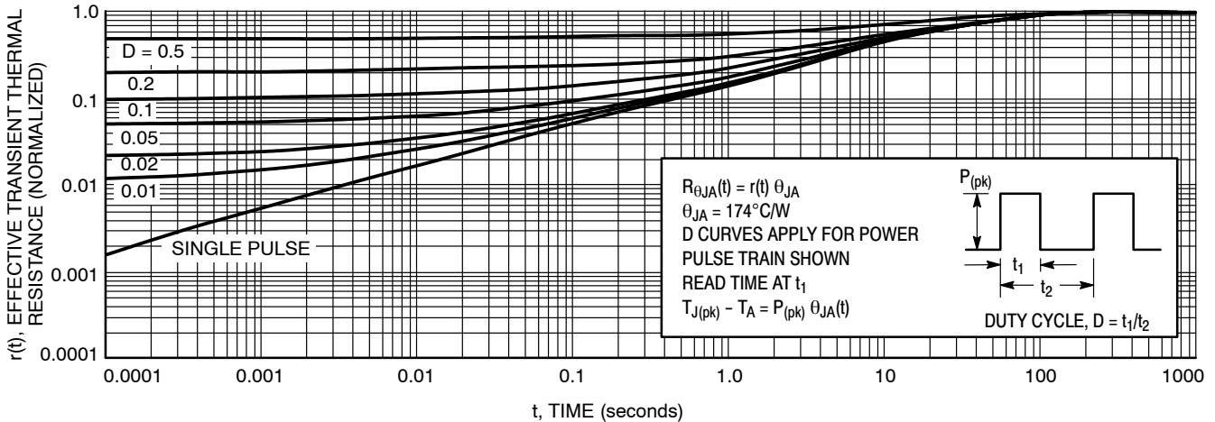
Figure 10. Thermal Response
