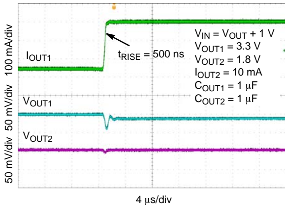
Figure 40. Load Transient Response – 1.8 V – Rising Edge, I_{OUT} = 50 \text{ mA} to 300 mA
