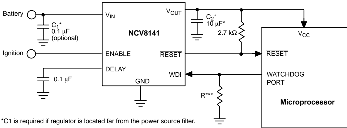
Figure 14. Application Diagram
